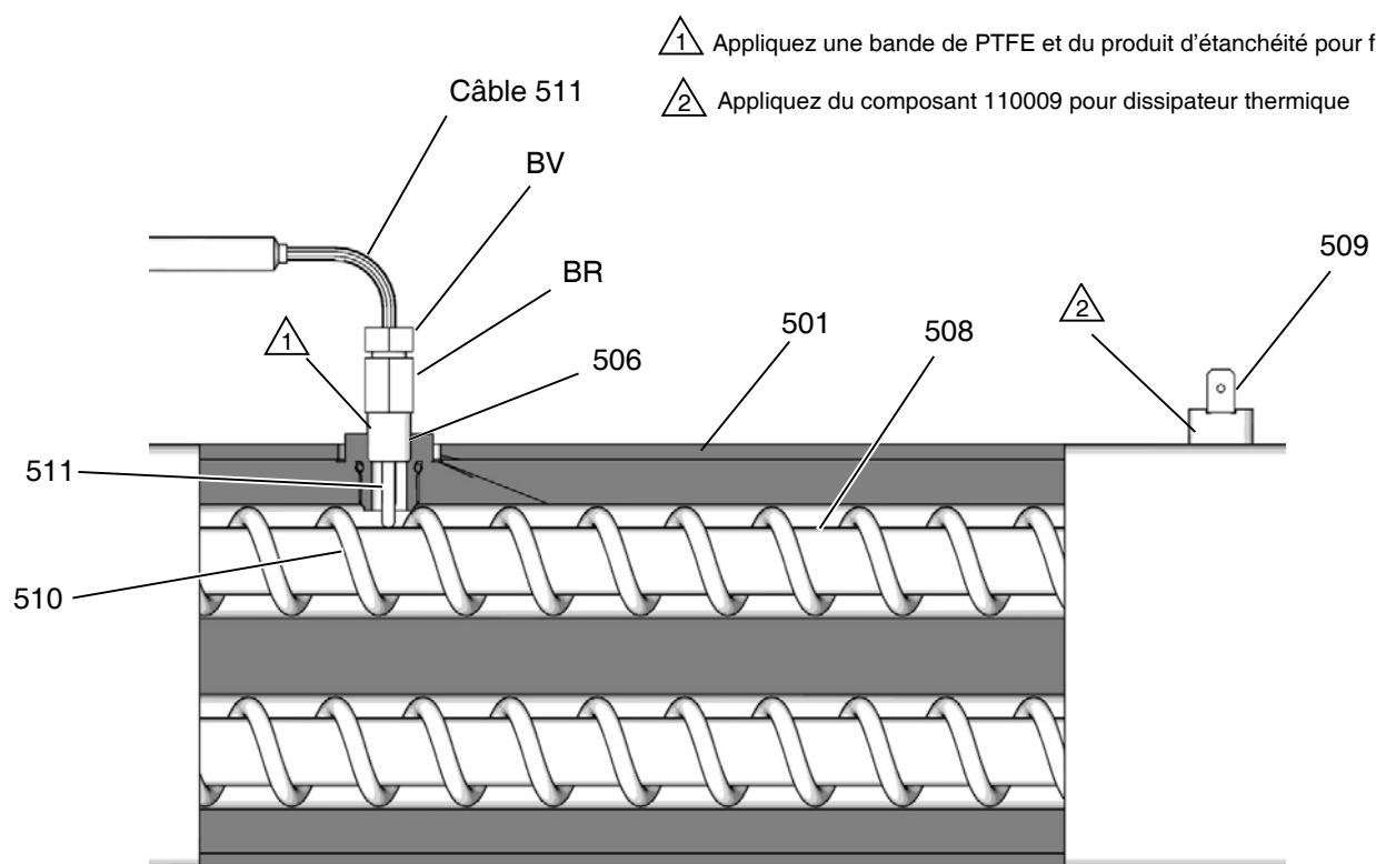
FIG. 69: Thermocouple
