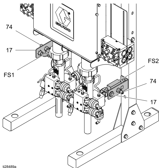
Figure 19 Raccords de solvant
