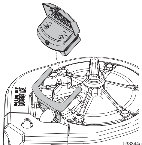
Fig. 5. Remove DataTrak from XL Air Motor
