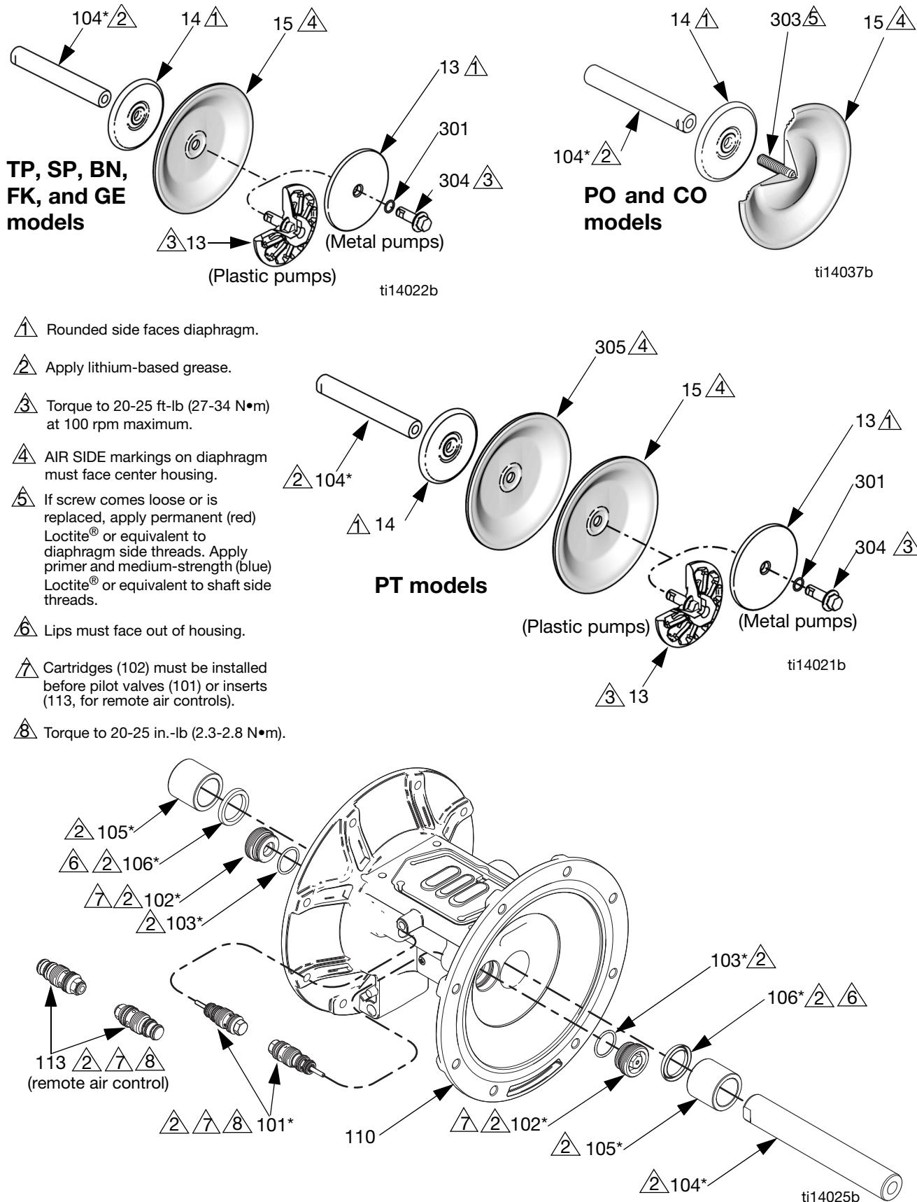
FIG. 8. Assemble diaphragms and center section
