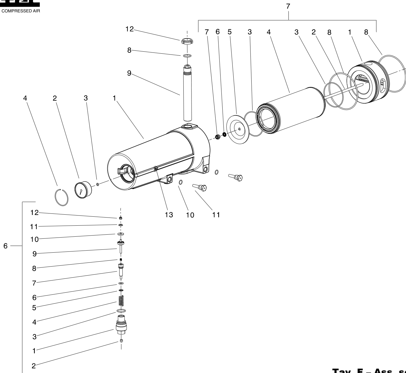
Tav. F – Ass. separatore aria-olio Air-oil separator assembly
