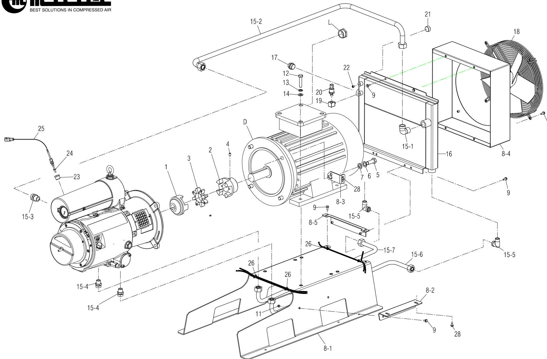
Tav. G – Gr. basamento - supporti Canopy base - support assembly
