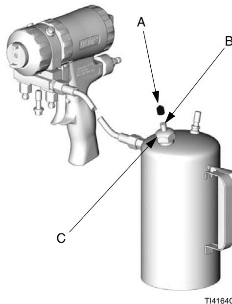
FIG. 4. Container Air Valve (Model 248139 Shown)
